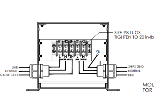
TYPICAL ELECTRICAL WIRING
